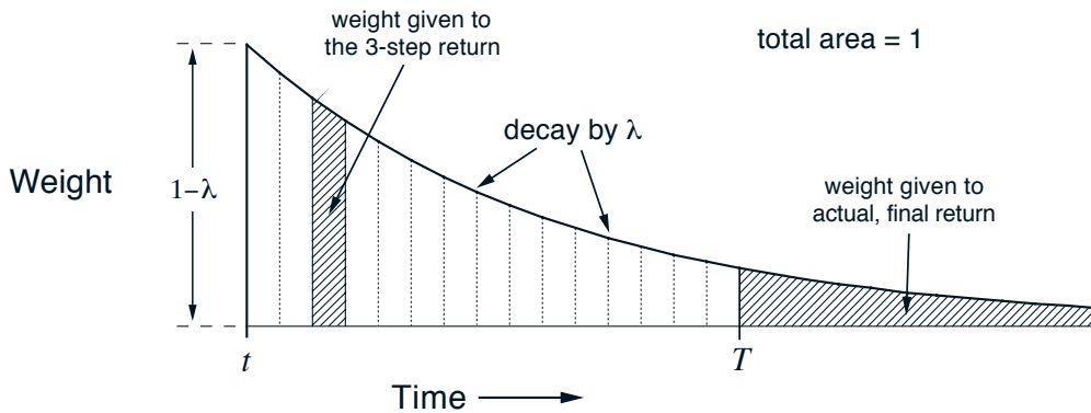
Figure 7.4: Weighting given in the \lambda -return to each of the n -step returns.
