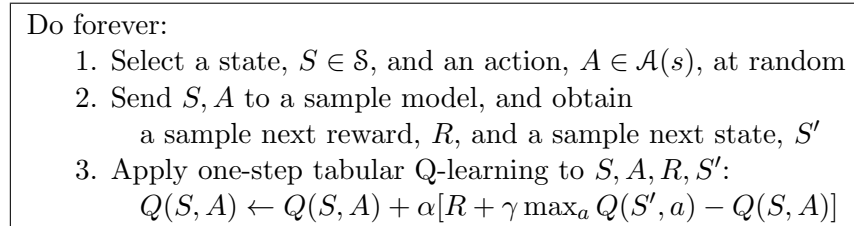
Figure 8.1: Random-sample one-step tabular Q-planning
